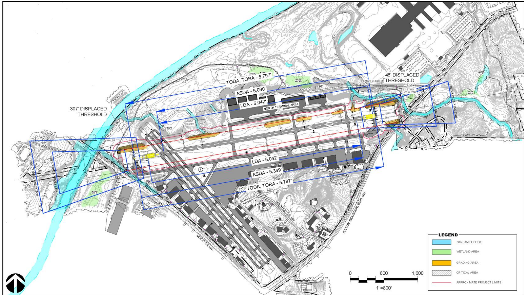
Figure 5-3: Alternative 1
