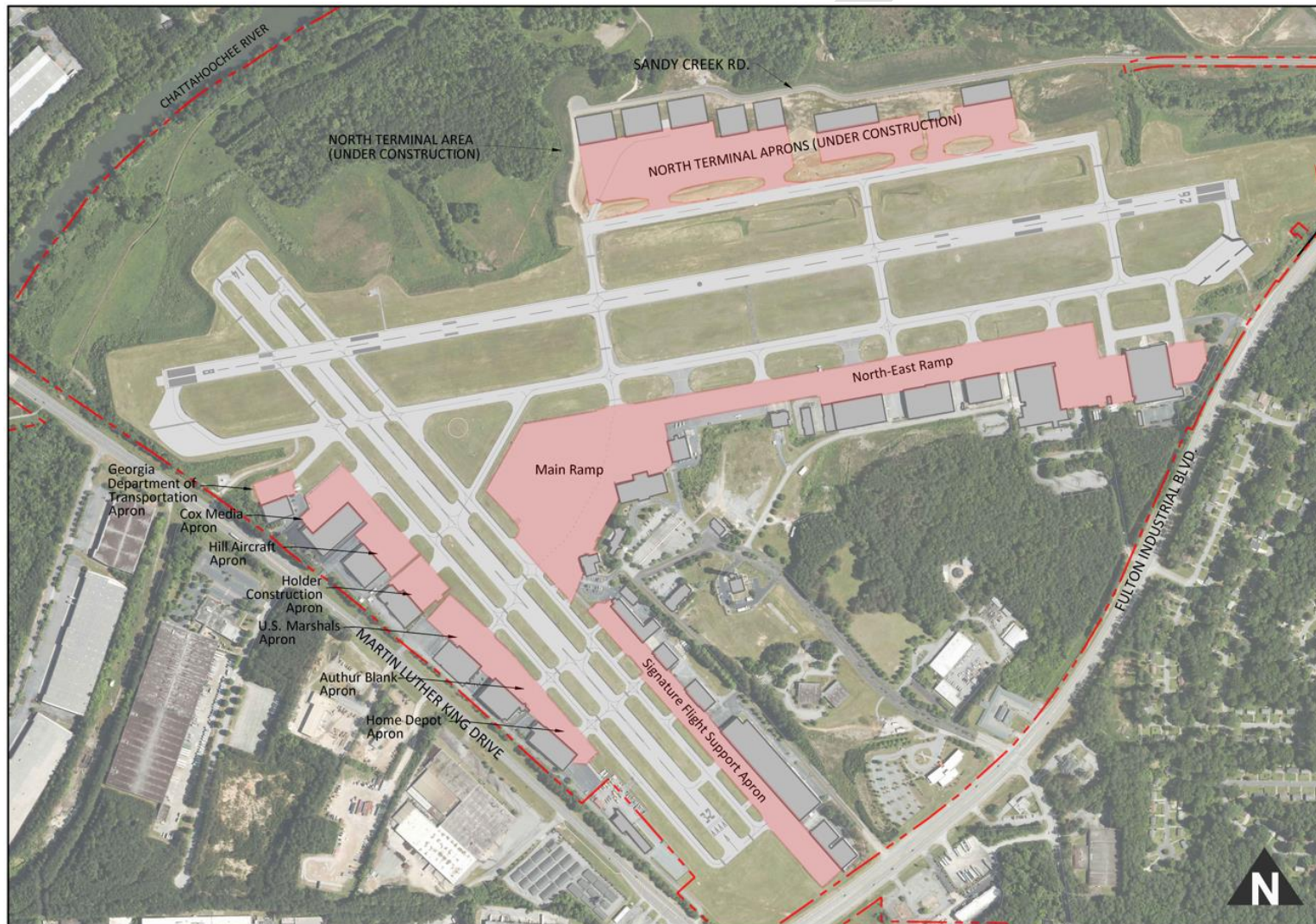
Figure 2-15: Apron Inventory
