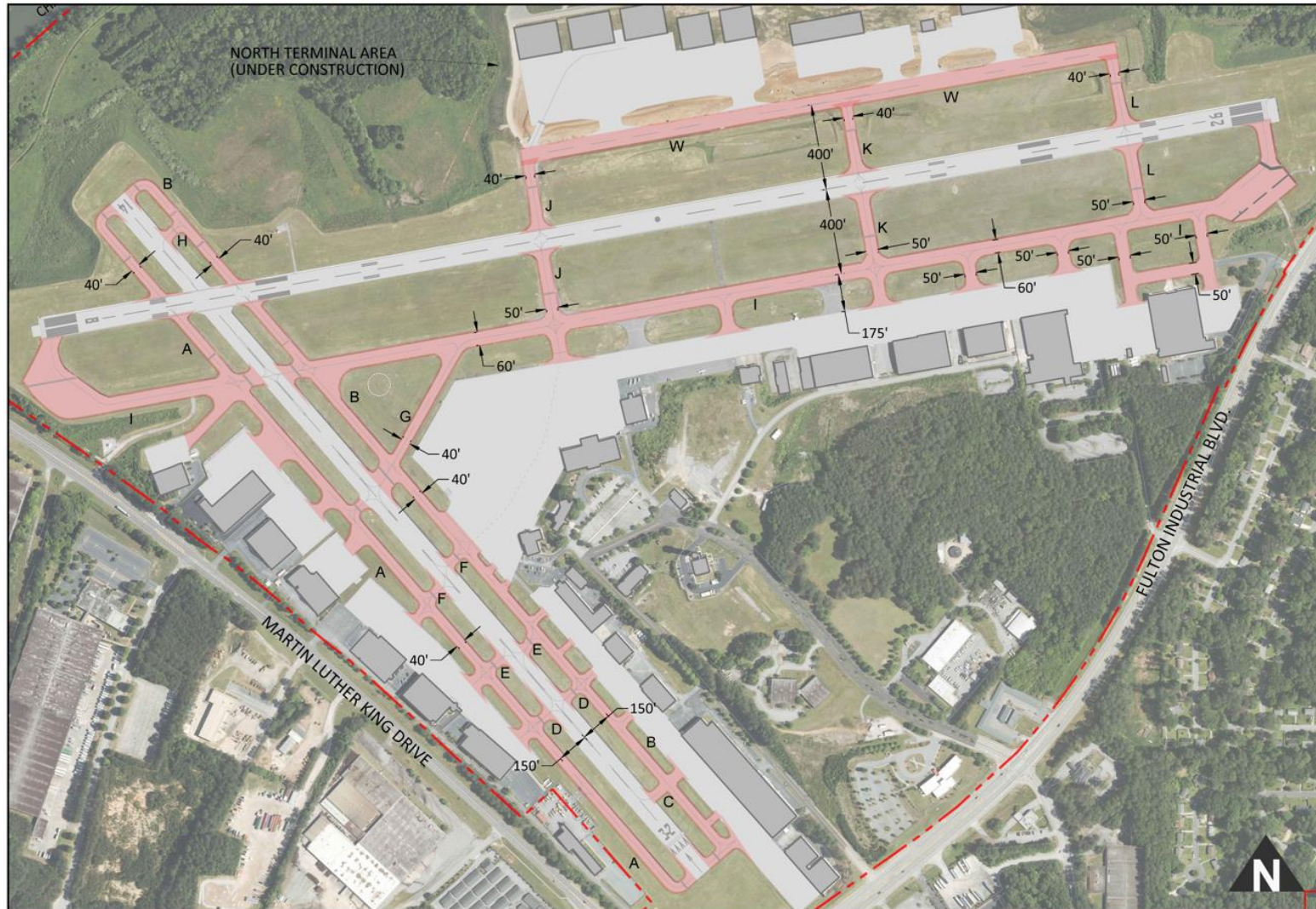
Figure 2-6: Taxiway System
