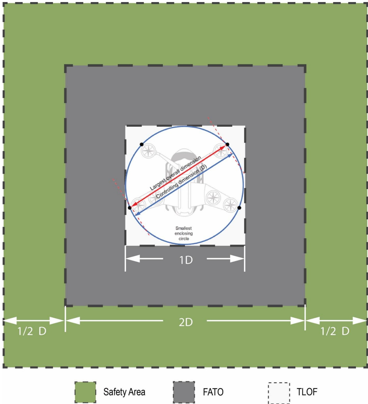
Figure 5-17: eVTOL Pad
