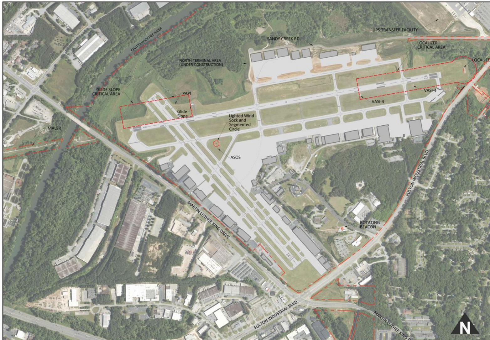
Figure 2-10: Navigational Aids
