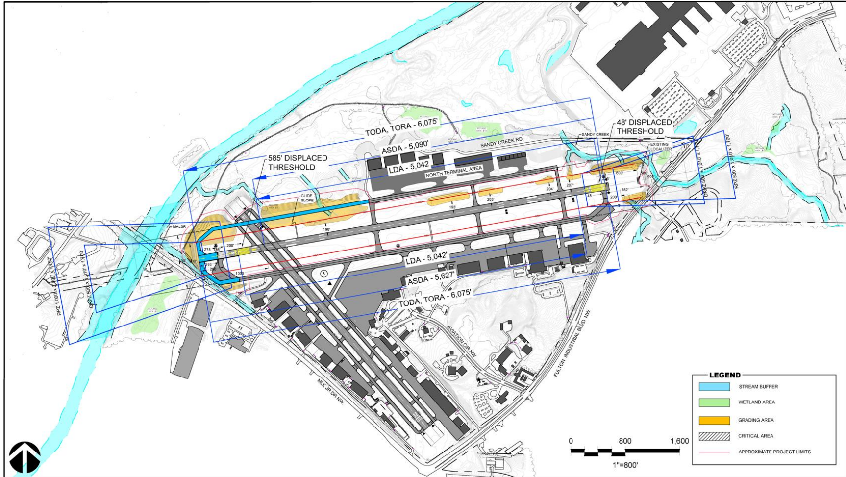
Figure 5-4: Alternative 2
