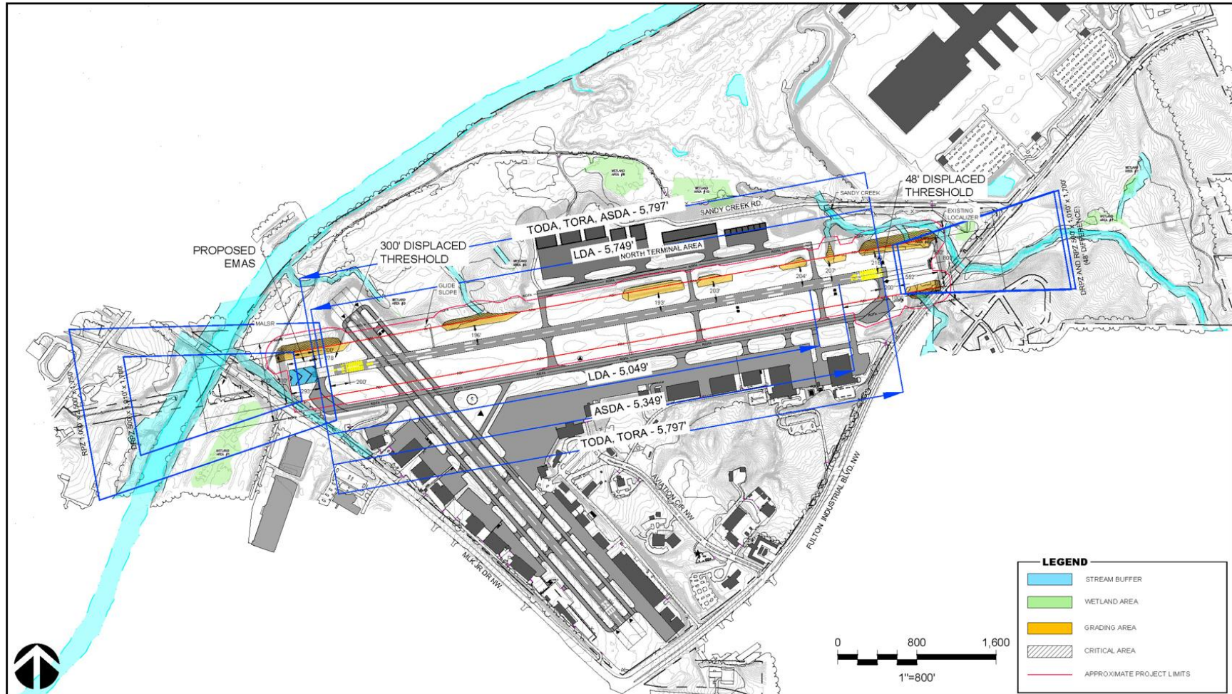
Figure 5-8: Alternative 6
